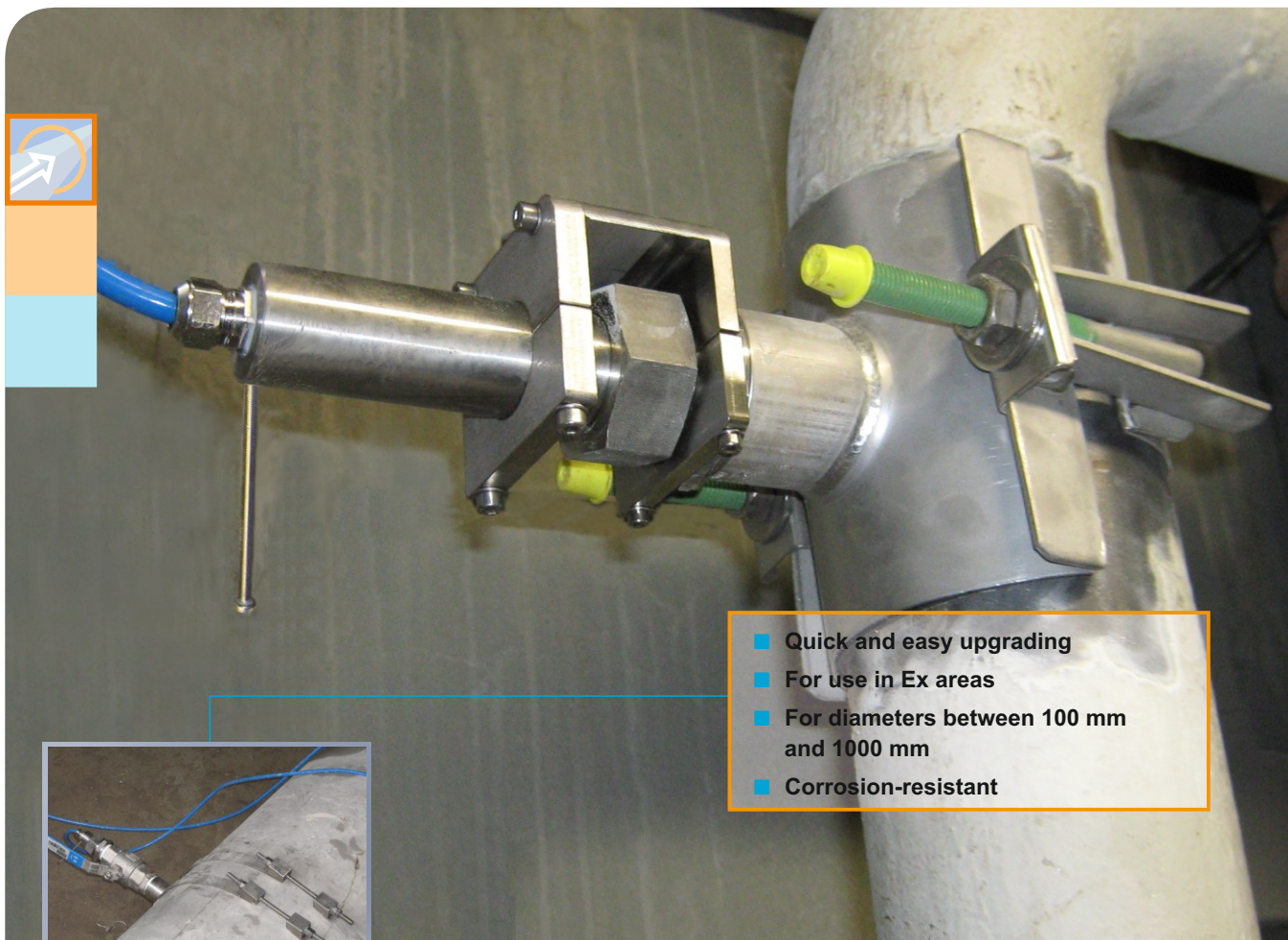
Tapping Saddle
